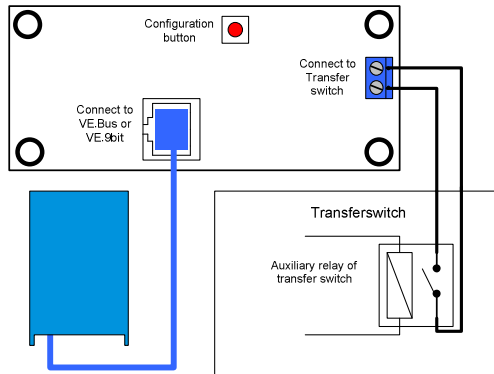
Figure 0.1 - Wiring diagram Digital Multi Control panel
